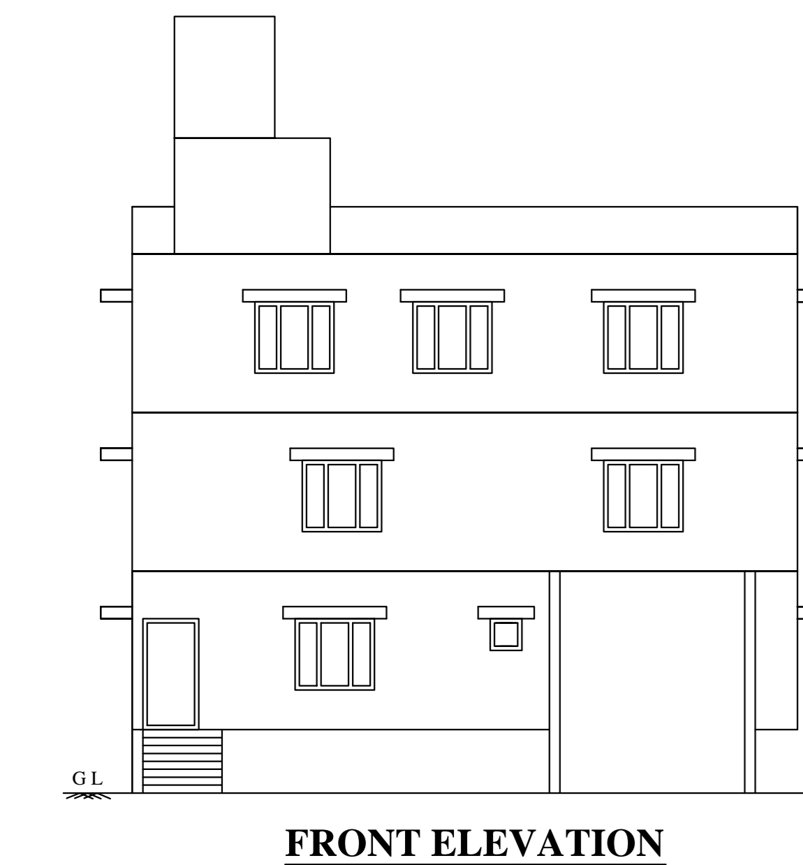
FRONT ELEVATION
